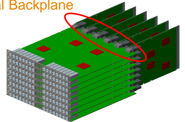
Orthogonal Backplane
